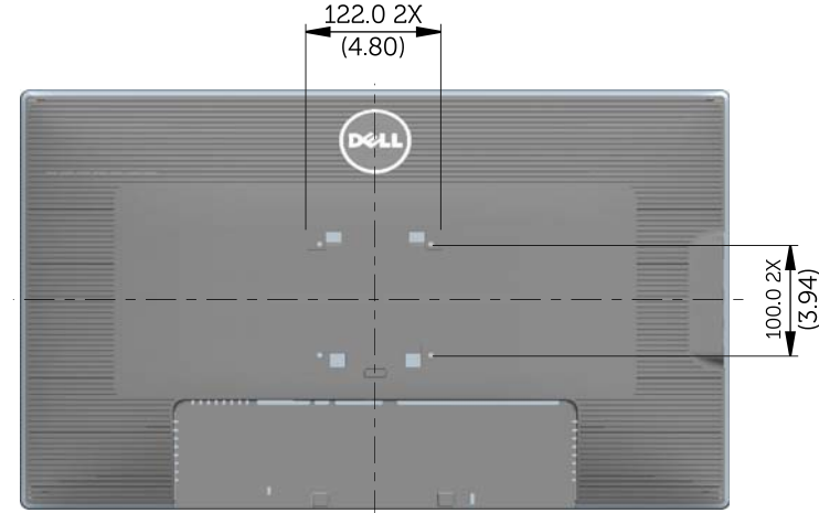
Back View of Monitor without stand
